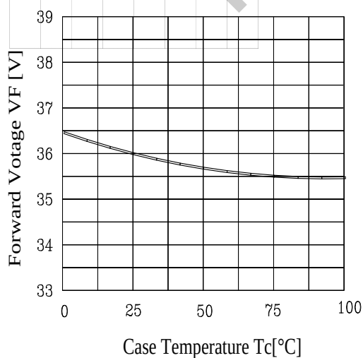
Case Temperature Vs. Forward Votage
