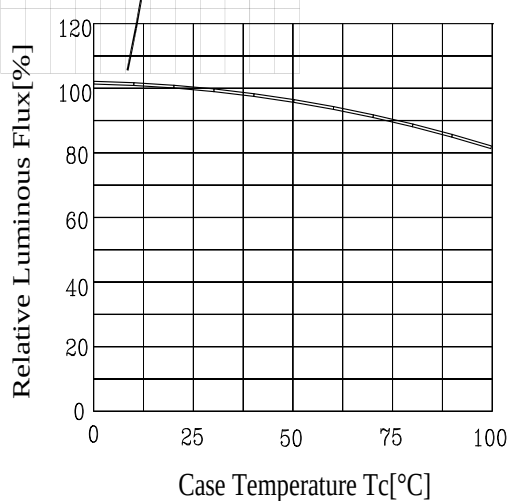
Case Temperature Vs. Relative Luminous Flux
