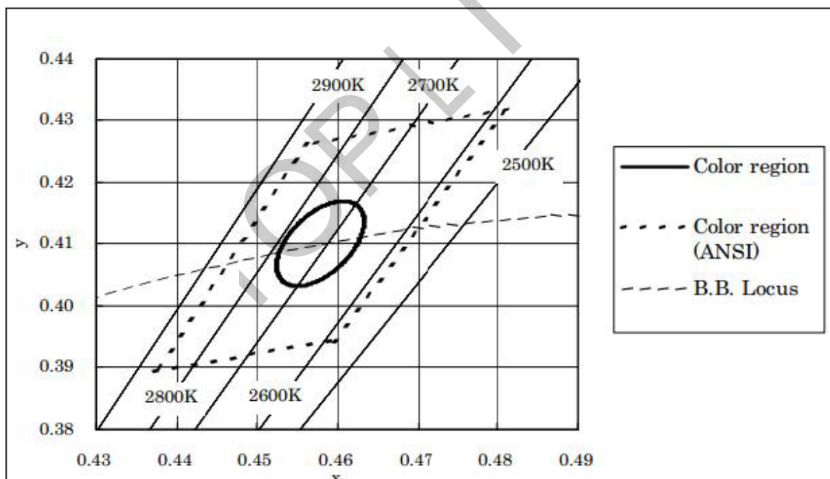
Chromaticity Diagram
