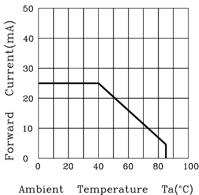
FORWARD CURRENT VS DERATING CURVE
